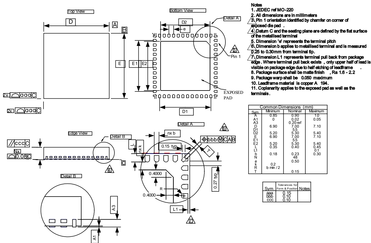
Figure 17. Package Drawing
